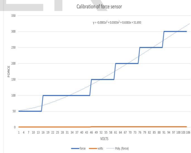
Figure 7. Calibration of FSR
