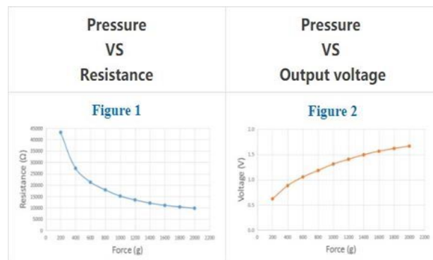
Figure 7. Relation between applied pressure and resistance of the sensor
